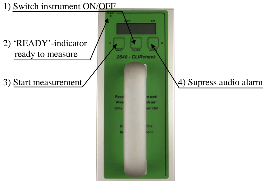
Fig. 1 Top view
