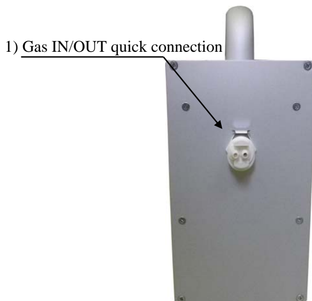
Fig. 2 Front View
